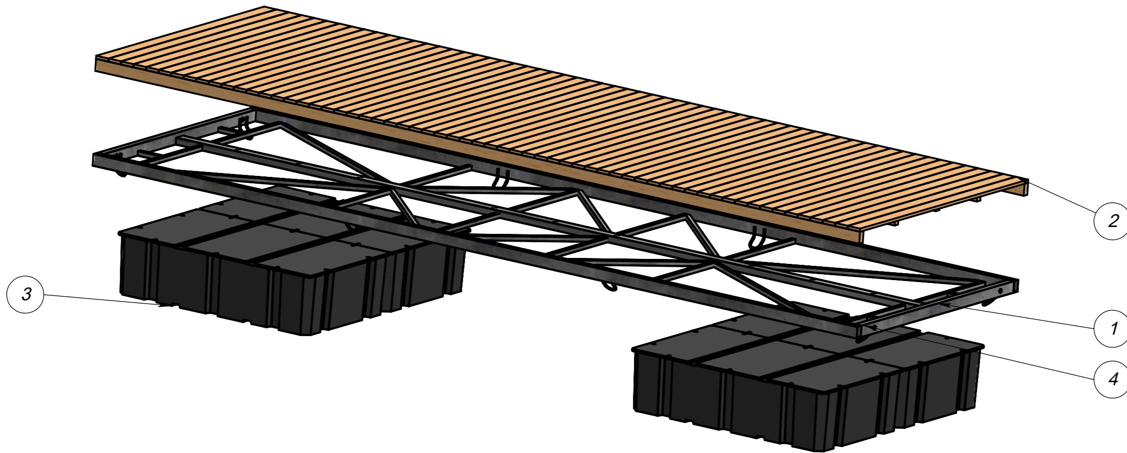
Steel frame-float connection
